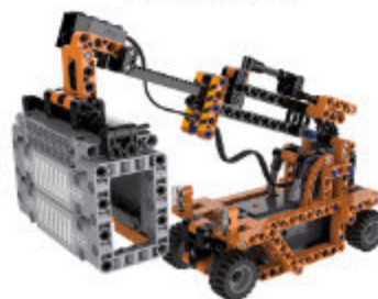
Container Loader
